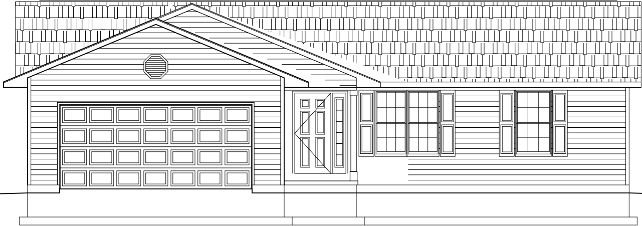
1 EAST ELEVATION A-1
